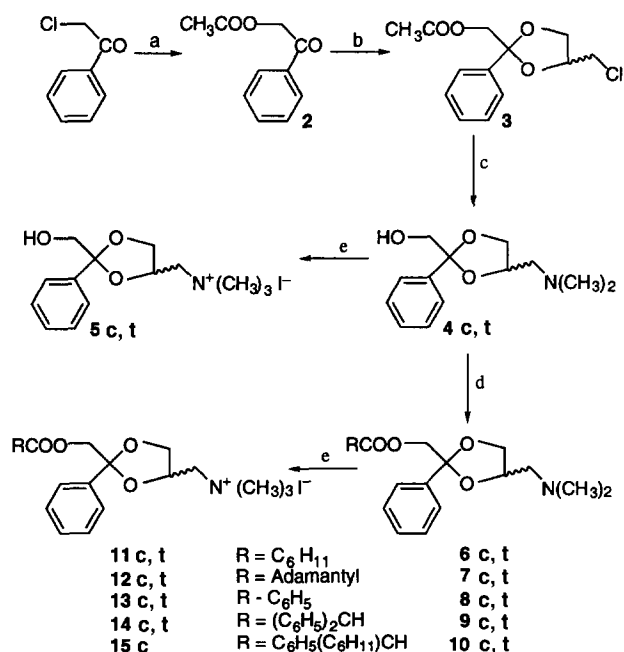
Scheme 1. (a) \text{CH}_3\text{COOK} , DMF, dicyclohexyl 18-crown ether-6, reflux; (b) an. \text{CH}_3\text{NO}_2 , 3-chloro-1,2-propanediol, triflic acid, molecular sieve 4 Å, reflux; (c) \text{HN}(\text{CH}_3)_3 , 100 °C; (d) \text{RCOCl} , an. pyridine, 0 °C to rt; (e) \text{CH}_3\text{I} , an. (\text{C}_2\text{H}_5)_2\text{O} . When the compound number is followed by c ( cis ) and t ( trans ), the two isomers have been separated.
