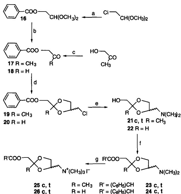
Scheme 2. (a) \text{C}_6\text{H}_5\text{COOK} , DMF, dicyclohexyl 18-crown ether-6, reflux; (b) THF, \text{H}_2\text{SO}_4 , reflux; (c) \text{C}_6\text{H}_5\text{COCl} , an. pyridine, –5 °C to ≥rt; (d) \text{C}_6\text{H}_5\text{CH}_3 , 3-chloro-1,2-propanediol, p -toluensulfonic acid, reflux; (e) \text{R}'\text{COCl} , an. pyridine, 0 °C to ≥rt; (f) \text{CH}_3\text{I} , (\text{C}_2\text{H}_5)_2\text{O} . When the compound number is followed by c ( cis ) and t ( trans ), the two isomers have been separated.
