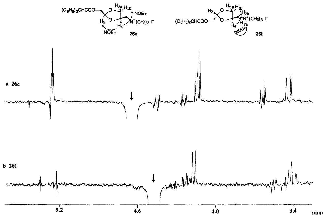
Figure 1. 1-D NOE difference spectra of compounds 26c (trace a) and 26t (trace b). The region between 3.3 and 5.5 ppm is shown.
